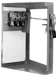
Complete Operating Mechanism — C361NE1
